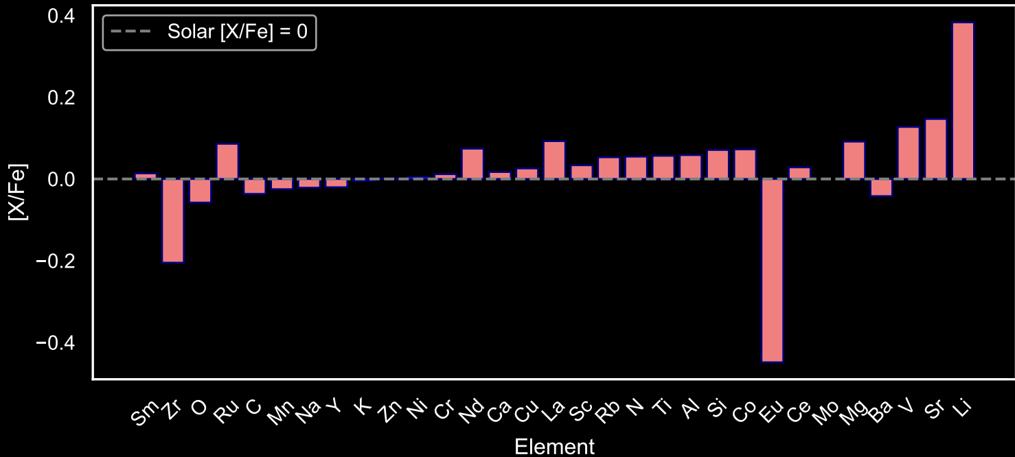
Abundance Pattern for GALAH Main Sequence Stars: Star Field [45] (N=111)
