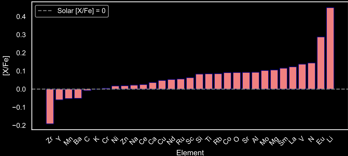
Abundance Pattern for GALAH Star Field [45] (N=218)
