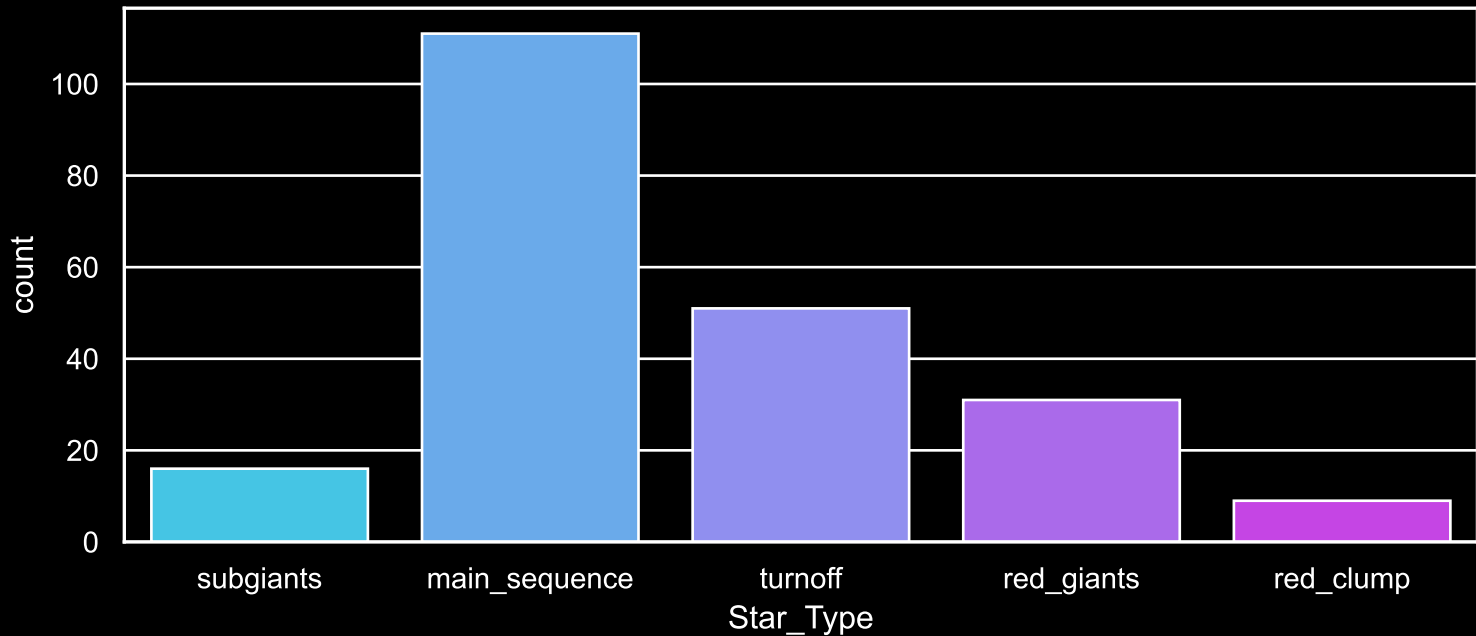
Field [45] Count plot of Star Type
