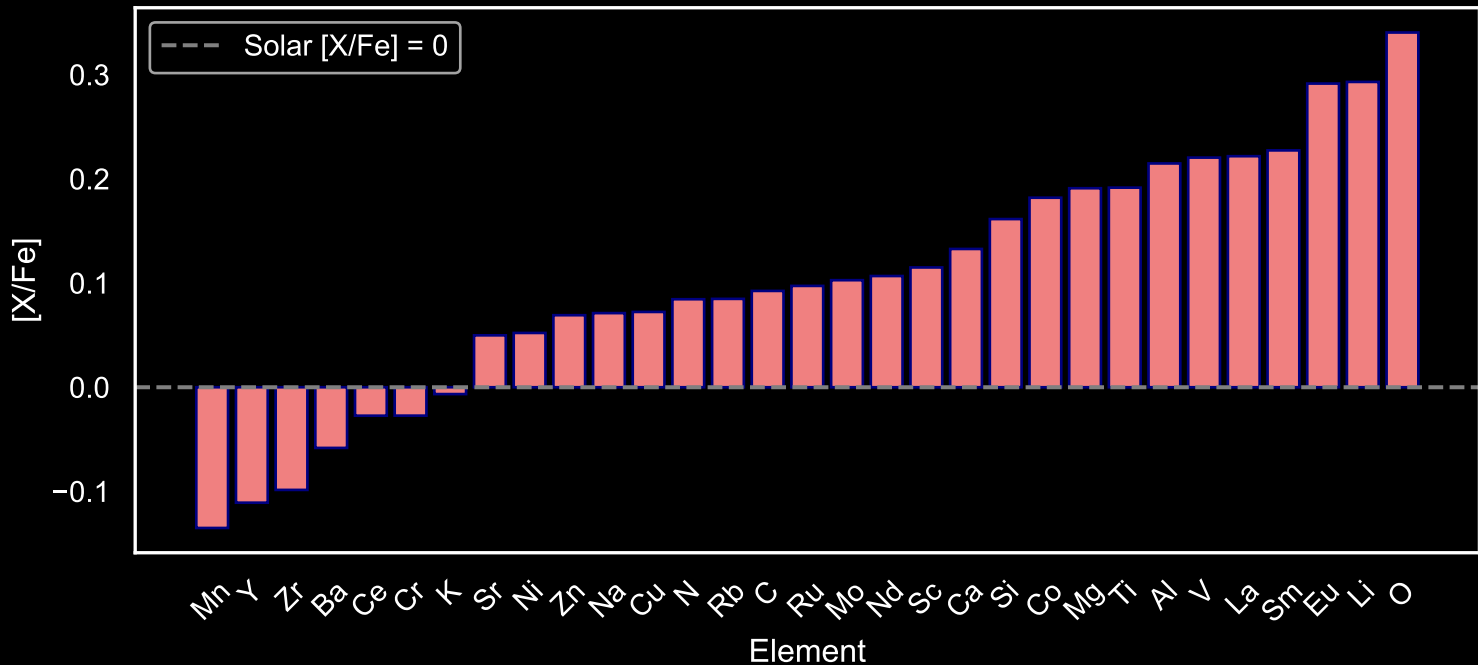
Abundance Pattern for GALAH Red Giants: Star Field [45] (N=40)
