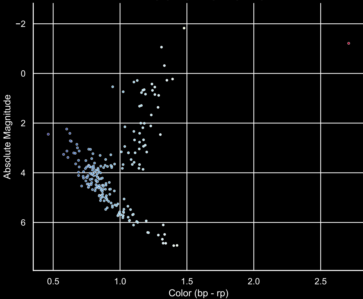
GALAH Hertzprung-Russel Diagram Field [45] Ra [347.88] Dec [-69.47]
